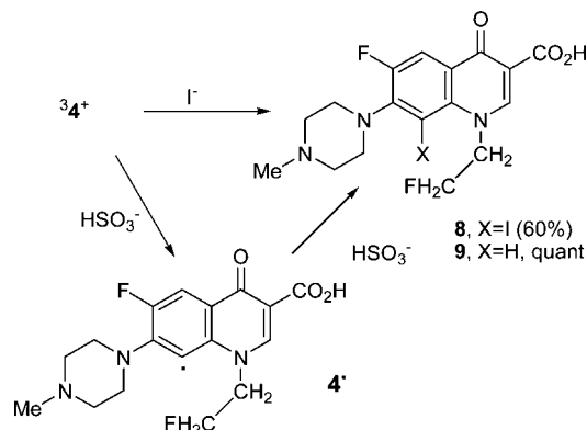
Scheme 3. Photochemistry of Fleroxacin ( 4 ) in the Presence of Iodide and Bisulfite
