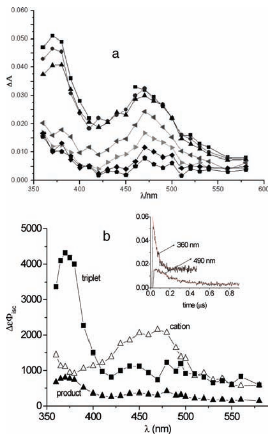
Figure 1. (a) Transients following excitation at 355 nm of a \text{N}_2\text{O} saturated 1.4 \times 10^{-4} M solution of 3 in 1.0 \times 10^{-3} M \text{NaHCO}_3 buffer of pH 7.2 at 25^\circ\text{C} .; upper trace, 40 ns, lower trace, 420 ns after the flash. (b) Calculated components by deconvolution of the previous transient absorption; for the attribution, see text. (Inset) Decays at 360 and 490 nm and biexponential best fit with \tau_1 = 41 ns and \tau_2 = 154 ns.
