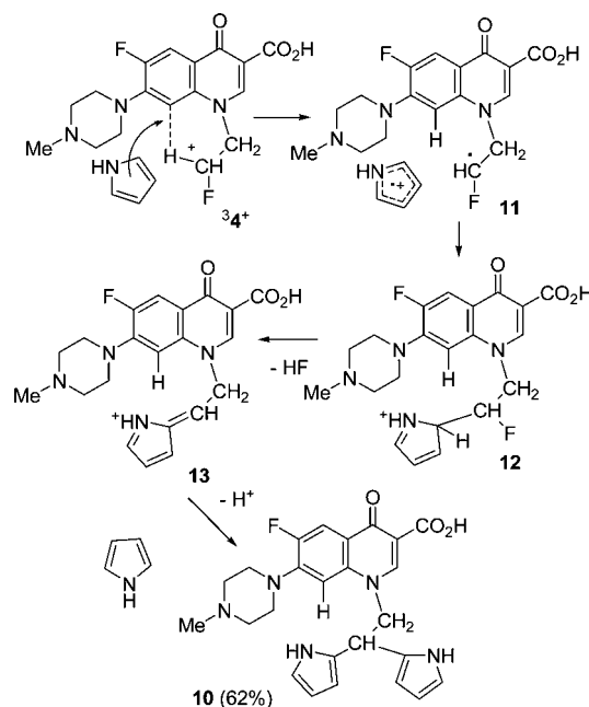
Scheme 4. Photochemistry of Fleroxacin ( 4 ) in the Presence of Pyrrole
