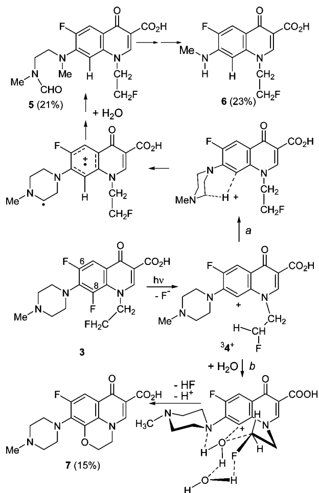
Scheme 2. Photochemical Reactions of Fleroxacin ( 3 ) in Water
